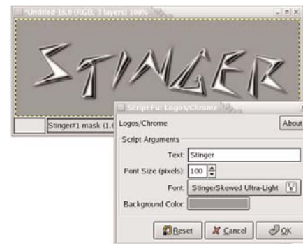
Figure 6. Font selections work basically the same in both versions. Getting fonts recognized by GIMP versions differs, however. GIMP 1.2 looks to the xfs server to provide fonts (try typing man xfs for help). GIMP 2.0 looks to FontConfig (see the fc-cache and fc-list commands for help here).
