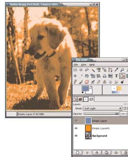
Figure 10. An alternative method to tinting an image is to use a layer that is fully colored and apply it using layer blend modes to the desaturated (but untinted) layer. This method has the advantage of not changing the desaturated layers' pixels and making use of compositing features of The GIMP to achieve the results you're after. Depending on the original layer, modes like Multiple, Overlay, Screen and Hard Light (among others) can help bring out detail in the image.
