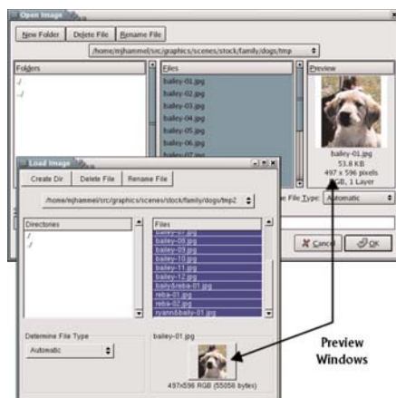
Figure 12. Both versions of The GIMP offer thumbnail previews. The previews are not generated without your request, but click on the preview frame, and the previews are generated for you. This image shows the File Selection dialog from GIMP 1.2 (foreground) and GIMP 2.0.
