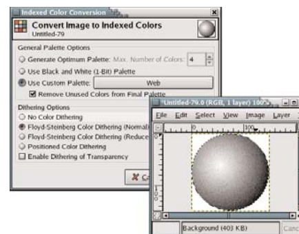
Figure 14. Once the noise is applied, you can map your image to Indexed. Select the Web custom palette. If the image doesn't look right, undo the mapping and the noise, and then apply an adjusted amount of noise and map again.
