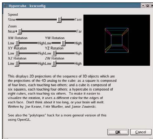
Figure 2. KDE Hypercube
